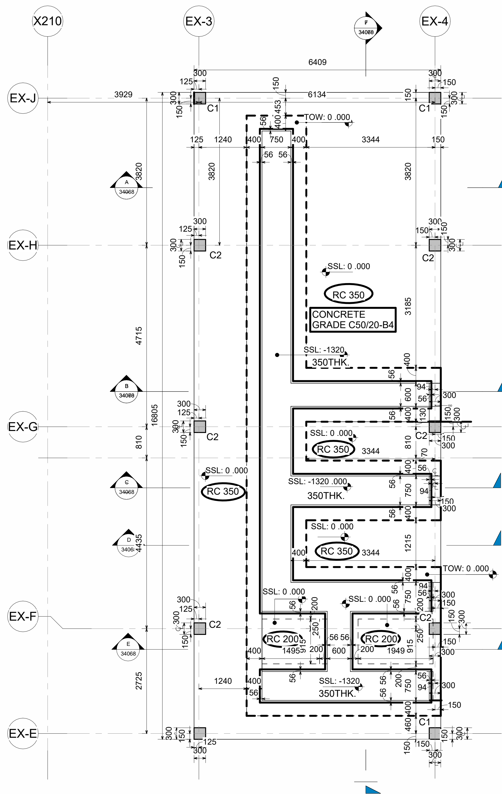
① GROUND FLOOR/RAFT FOUNDATION PLAN 1 : 50
