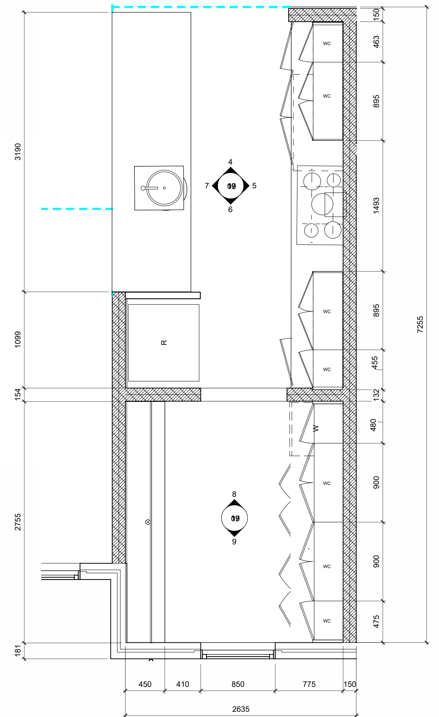
9 KITCHEN PLAN 1 : 25
