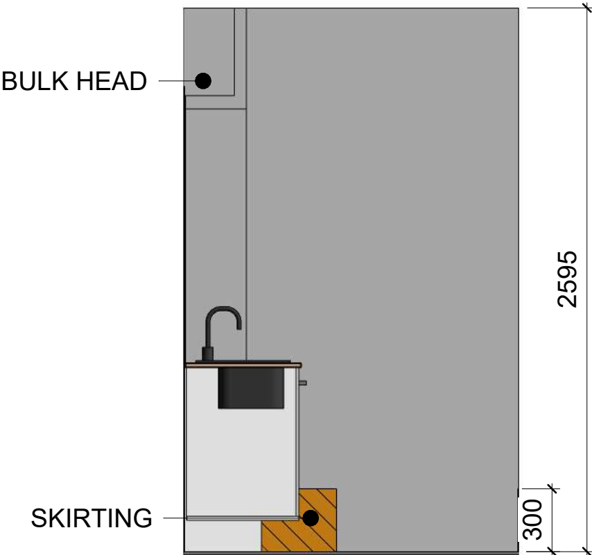
ELEVATION B1 1 : 25
