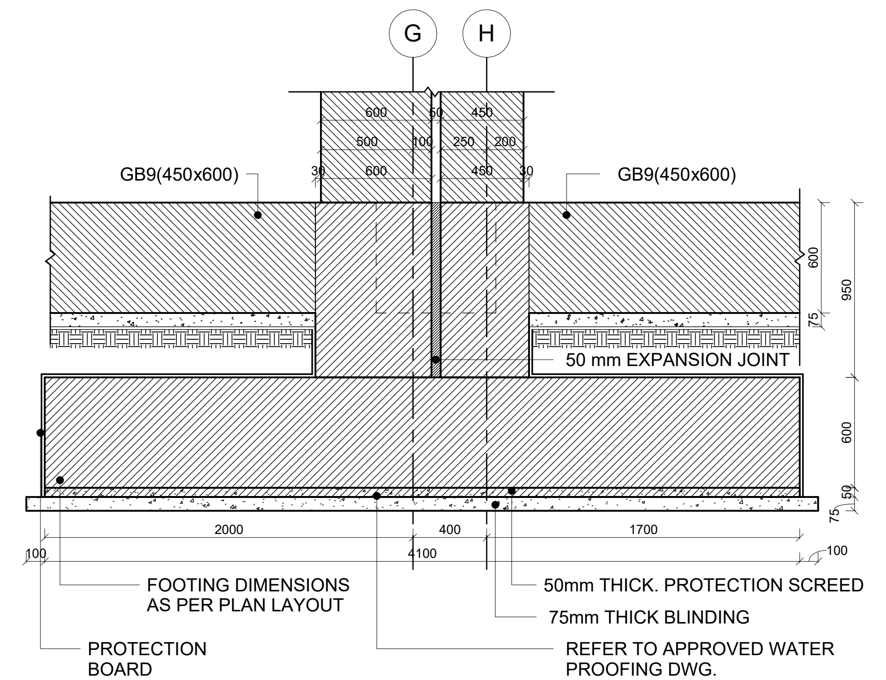
7 SECTION-07 (F5) DETAIL 1 : 20
